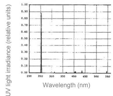
Emission spectrum for UV-C germicidal tube
