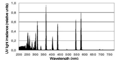
Emission spectrum for mercury UV bulb
